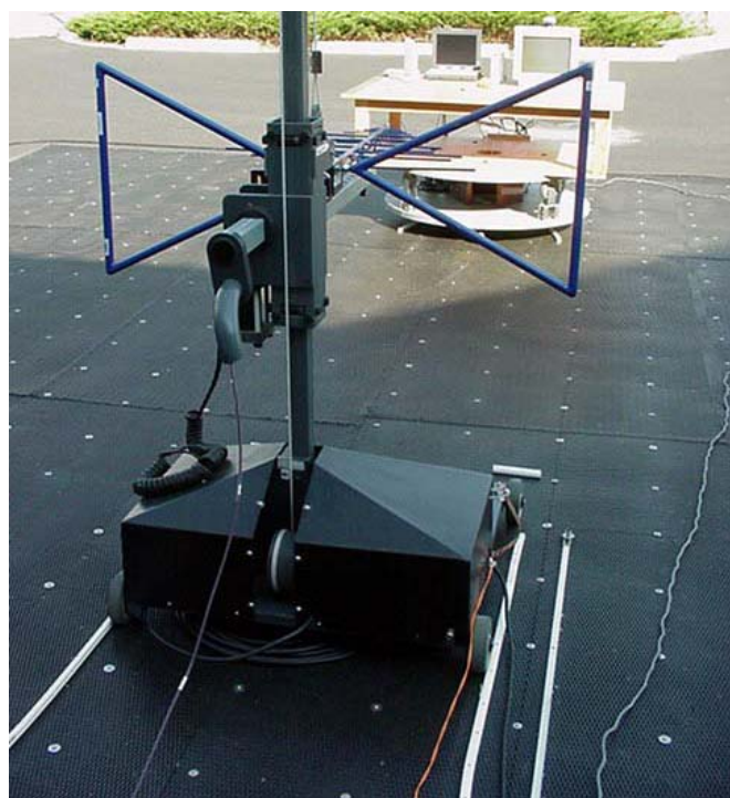
Photograph F-3 - Front of Radiated Emission Configuration
