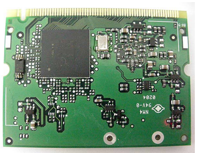
Photograph A-13 - Back of Intel Pro 2200BG Mini-PCI WLAN Card without Label
