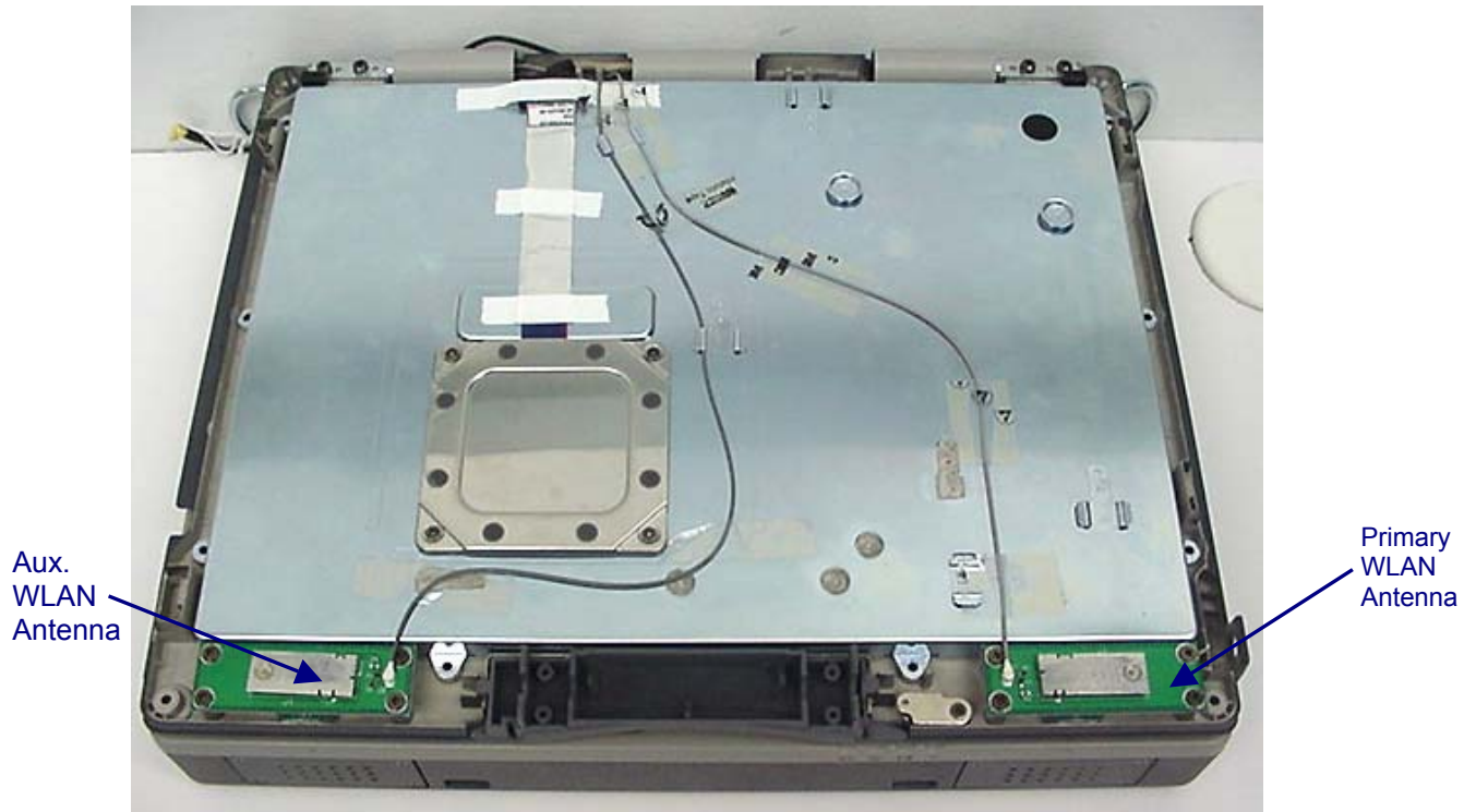
Photograph A-17 - Distance Between Integrated WLAN Antennas
