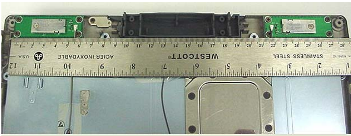
Photograph A-17 - Distance Between Integrated WLAN Antennas
