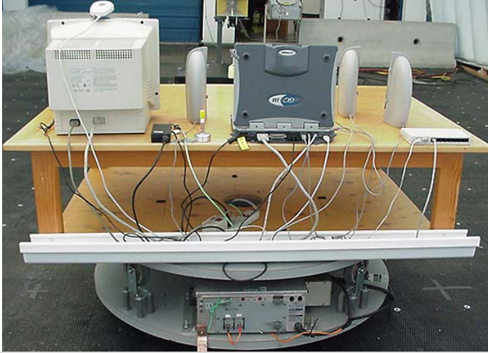
Photograph E.7-5 - Back of Radiated Emission Setup with attached swivel dipole antenna
