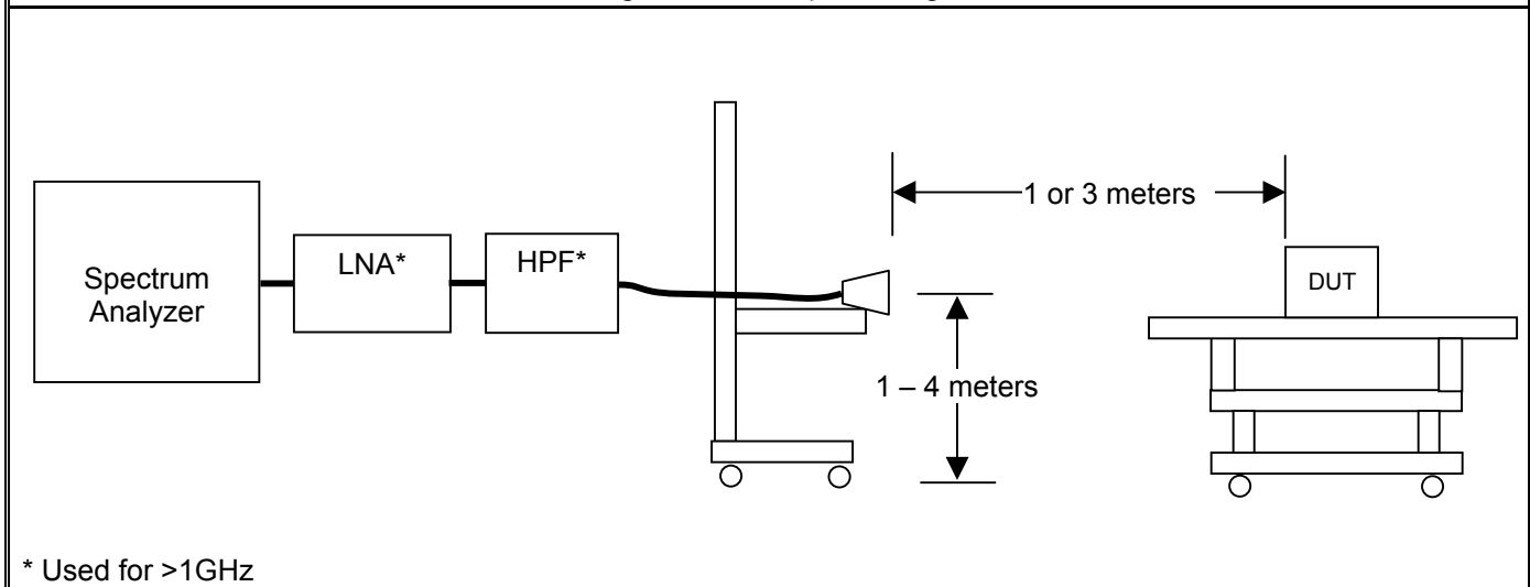
Figure I-1 - Setup Drawing
