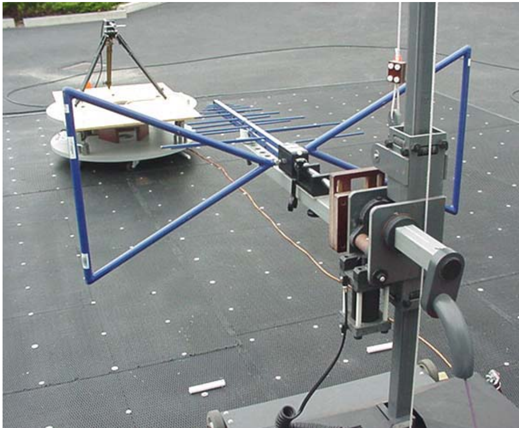
Substitution Dipole antenna
