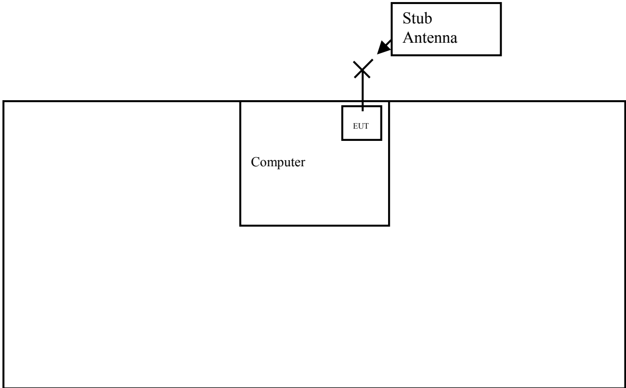
FIGURE 1: TESTED CONFIGURATION
