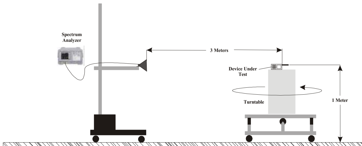
Figure 1. Radiated Measurement Test Setup Diagram
