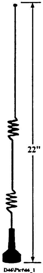
Figure 1: 46-0066-001 Antenna dimensions (For Reference Only)
