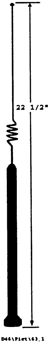
Figure 1: 46-0063-001 Antenna dimensions (For Reference Only)
