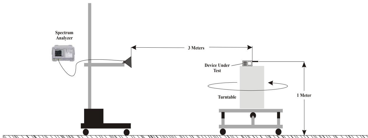
Figure 1. Radiated Measurement Test Setup Diagram
