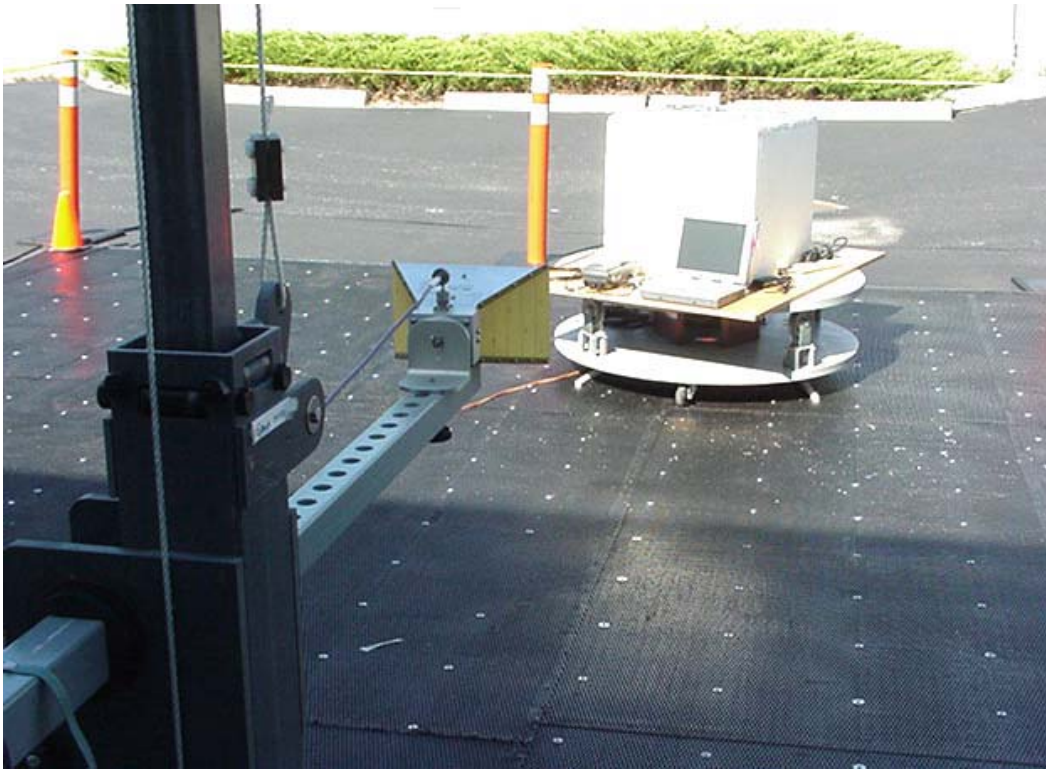
PCS Band with Horn Receive Antenna
