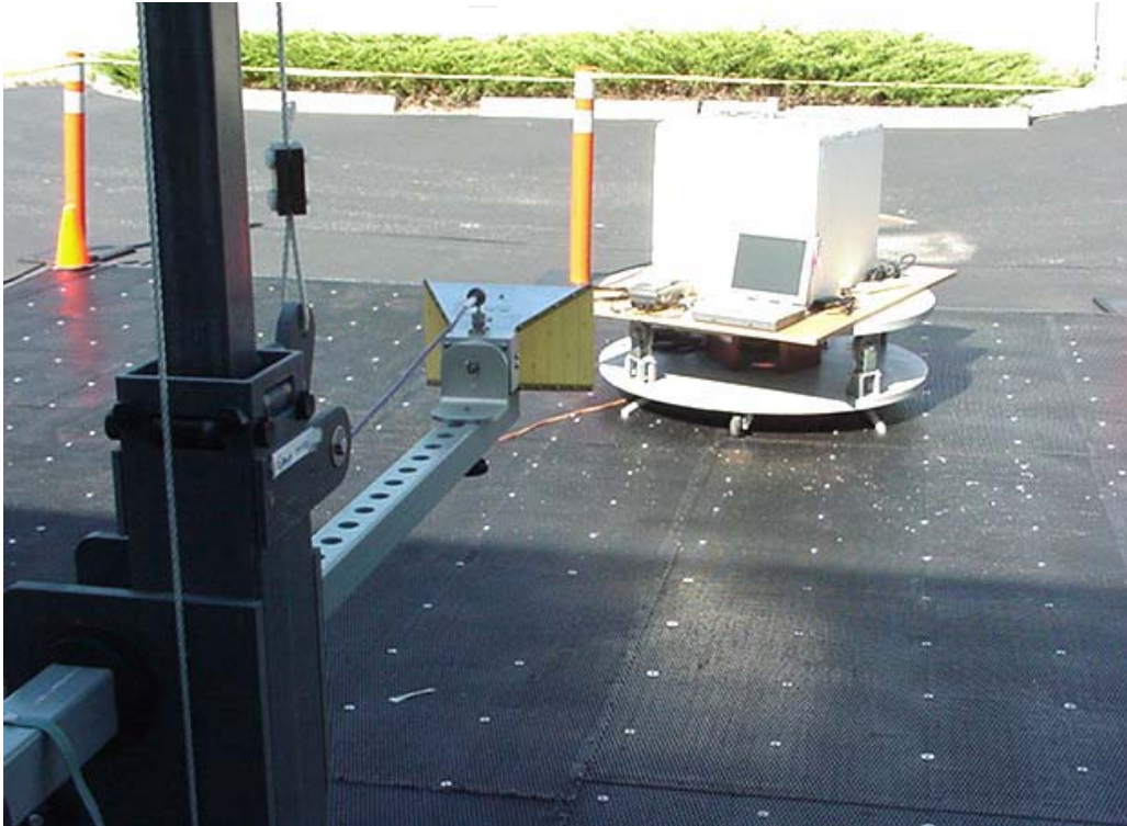
DUT with IX100X Vehicle Cradle & MaxRad 3 dBi Gain Vehicle-Mount Antenna (P/N: WMLPVDB800/1900)
