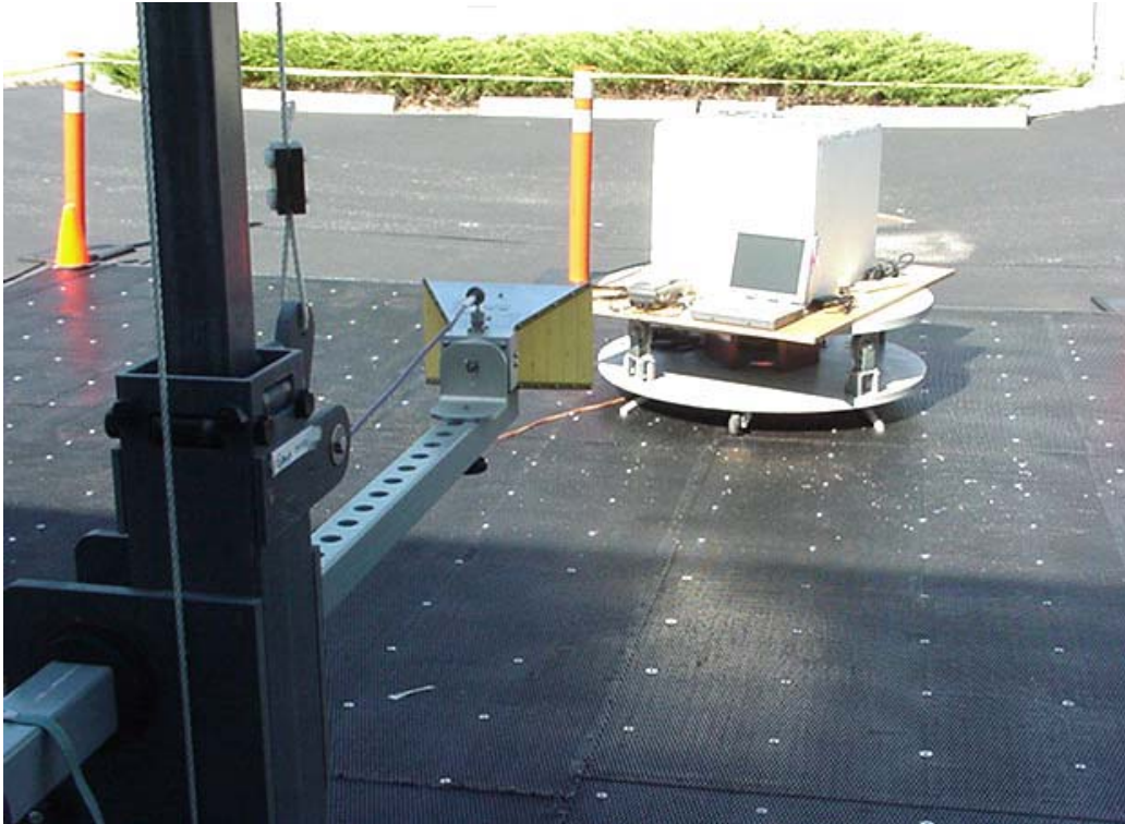
With Horn Receive Antenna
