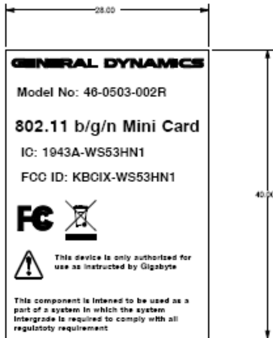
Figure 1: Label Drawing
