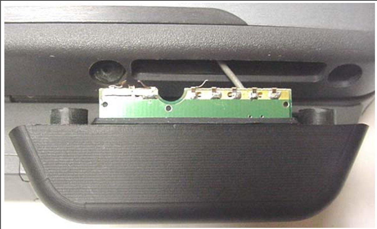
IX-MC5725 Antenna and Housing - Top View
