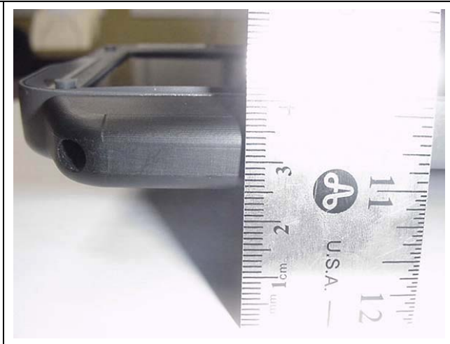
2.5 cm Antenna Spacing - LCD Display Fully Extended (IX750 PC with Extended Capacity Lithium-ion Battery)
