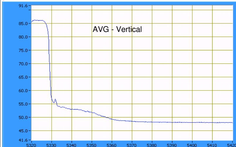
Log scale - scaling assumes units are dB units with correction factor applied (36.6 @ 5370.0 MHz)
