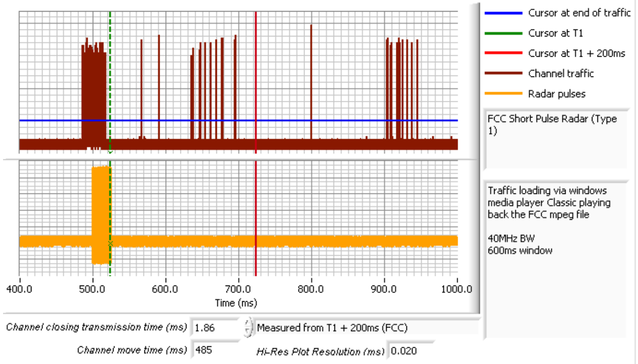
Figure 6 Close-Up of Transmissions Occurring More Than 200ms After The End of Radar (40MHz BW)
