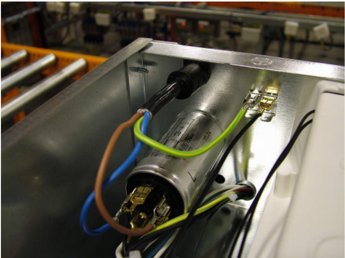
Mains filter
