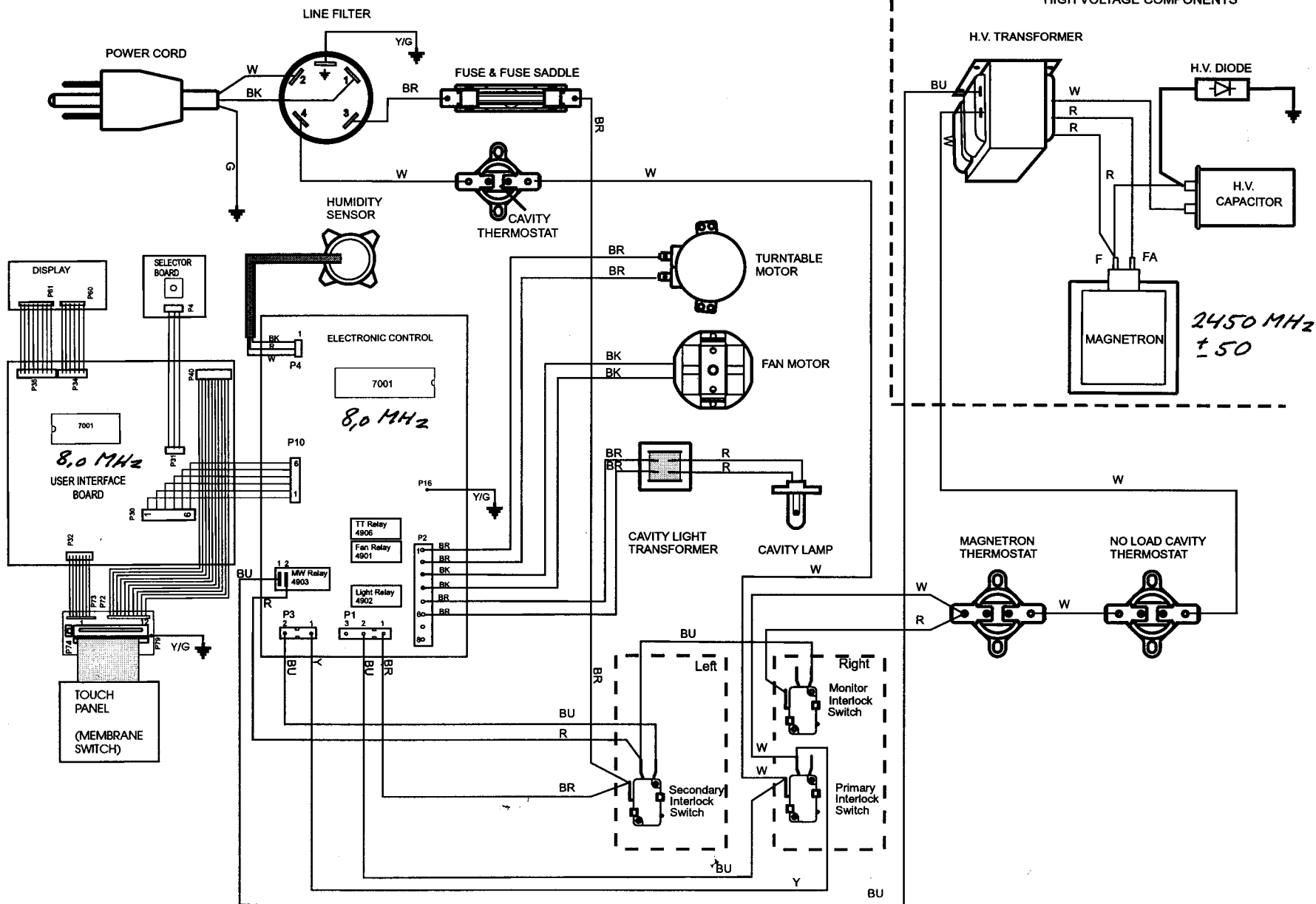
Pictorial Diagram
