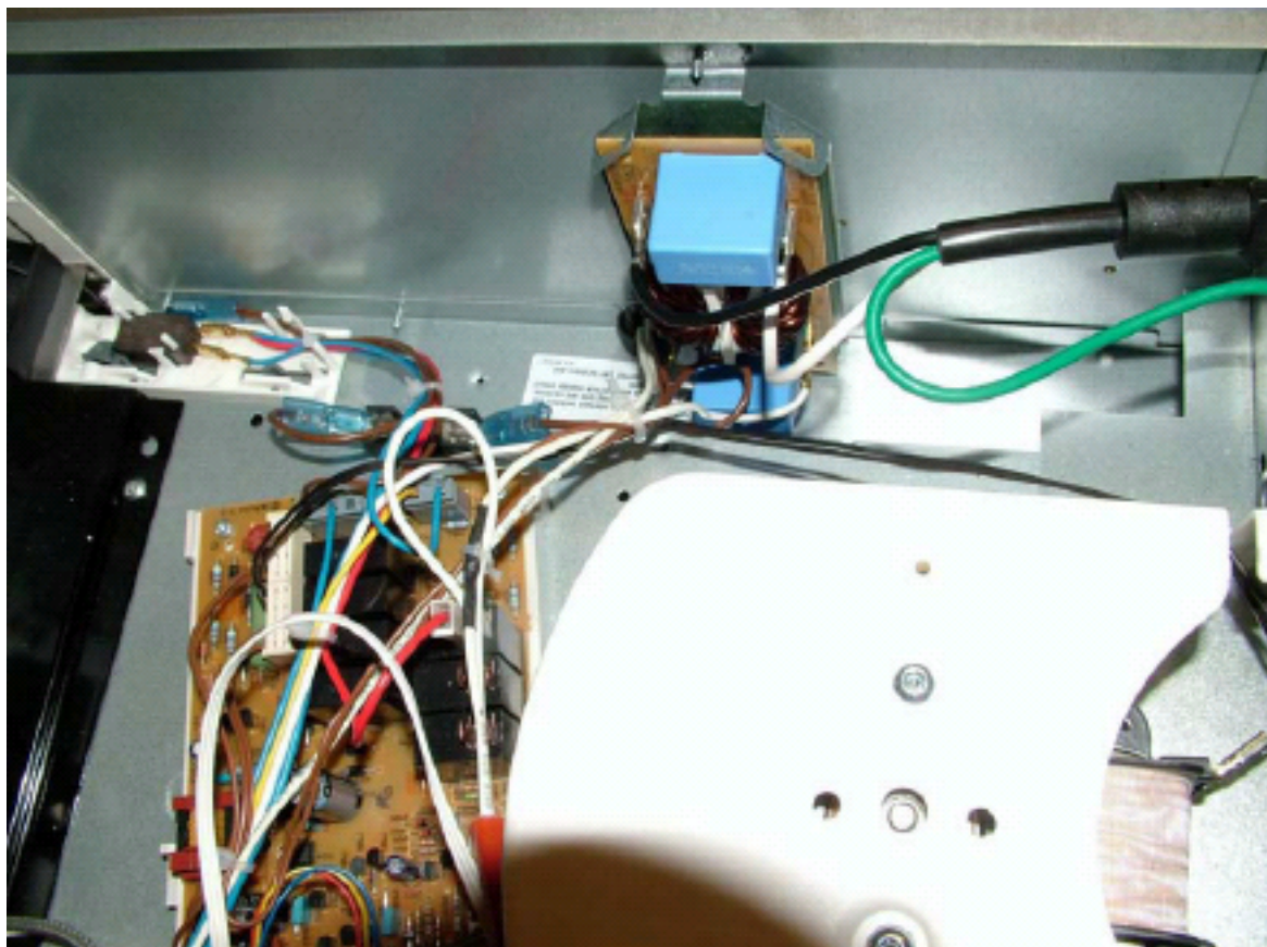
Mains filter
