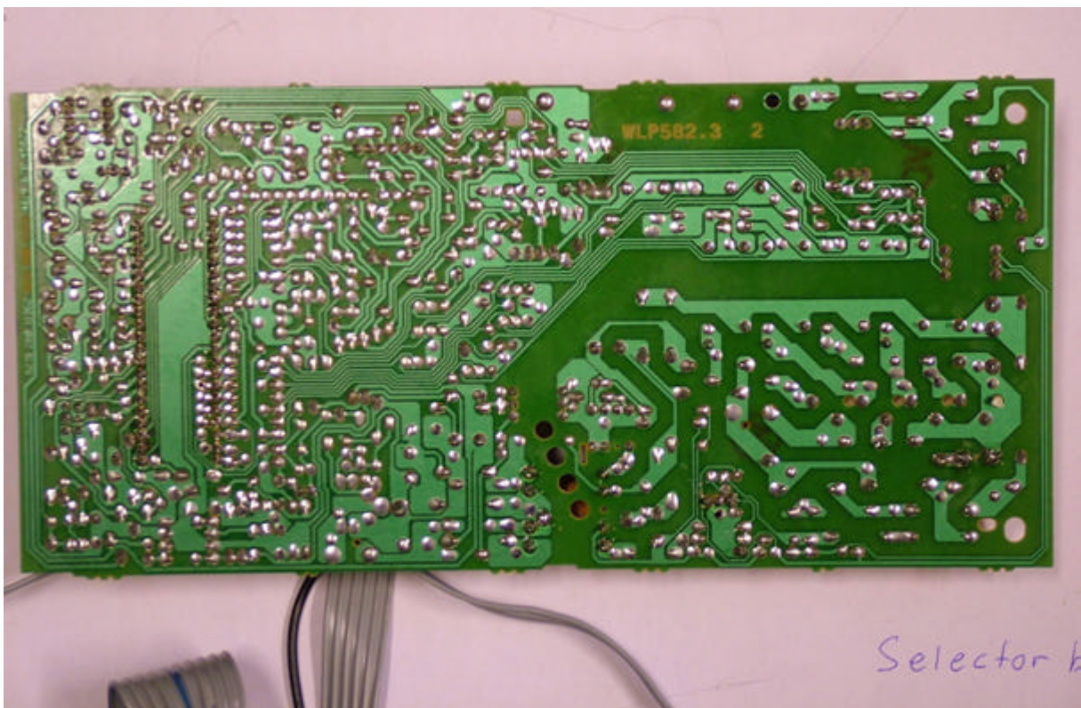
Power board
