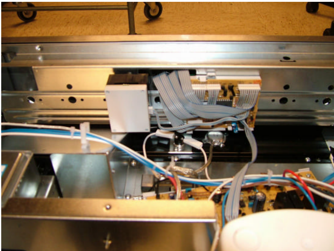
Control board
