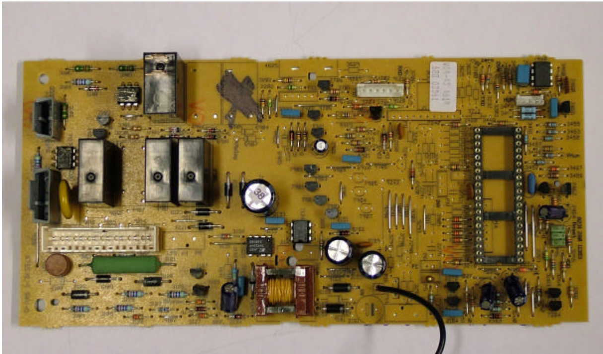
Power board
