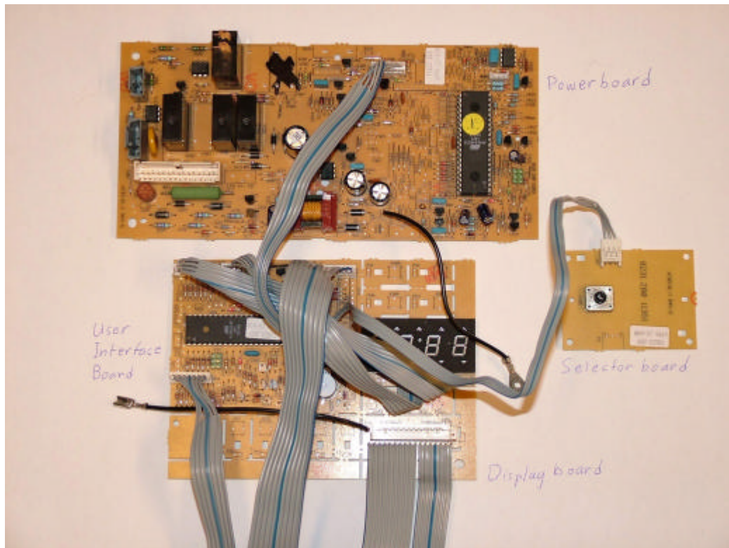
PCB's
