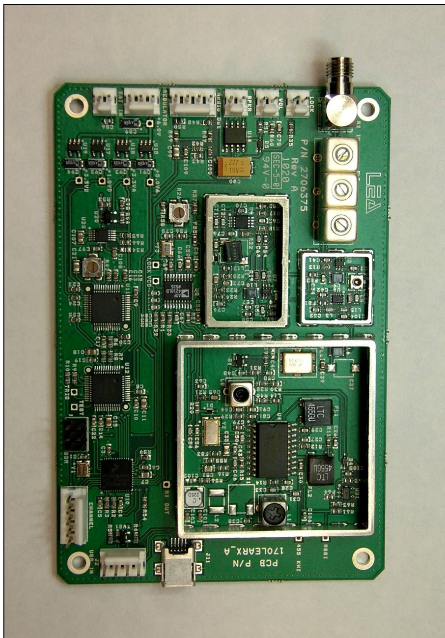
Assembly P/N 2706375 Rev A Top View with Shields Removed
