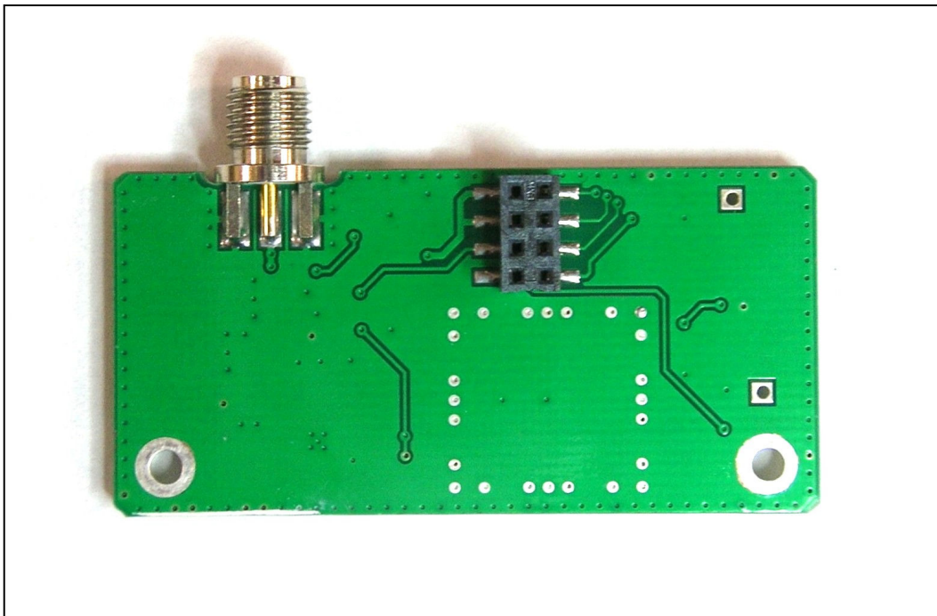
Assembly P/N 2705300-2 Rev A Bottom View
