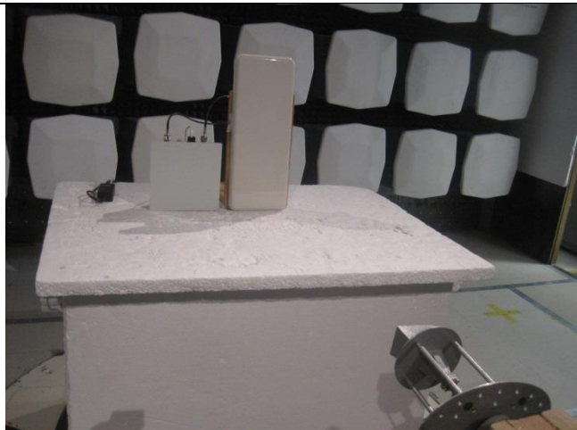
Radiated Spurious Emissions 18-40GHz (16dBi Ant) – Front View
