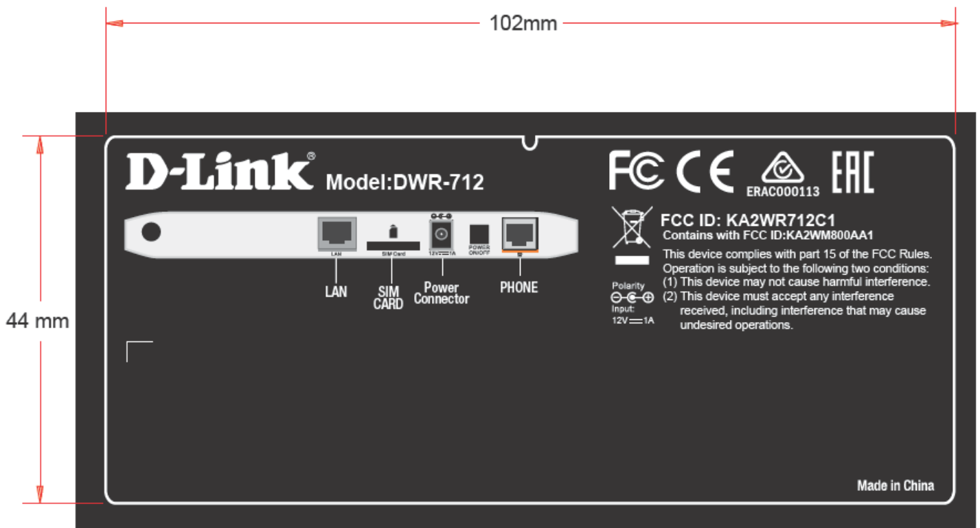
Label location
