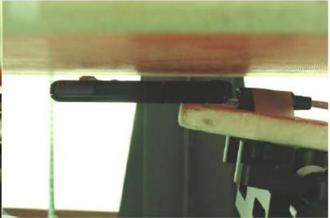
USB Cable Plug-in for USB Configuration 2 (Horizontal Down with Phantom 5 mm Gap)
