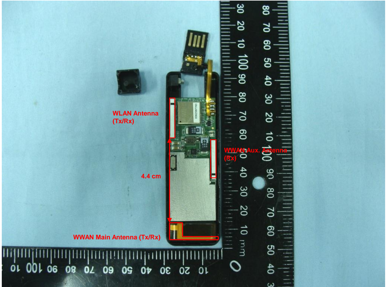
Antenna Location
