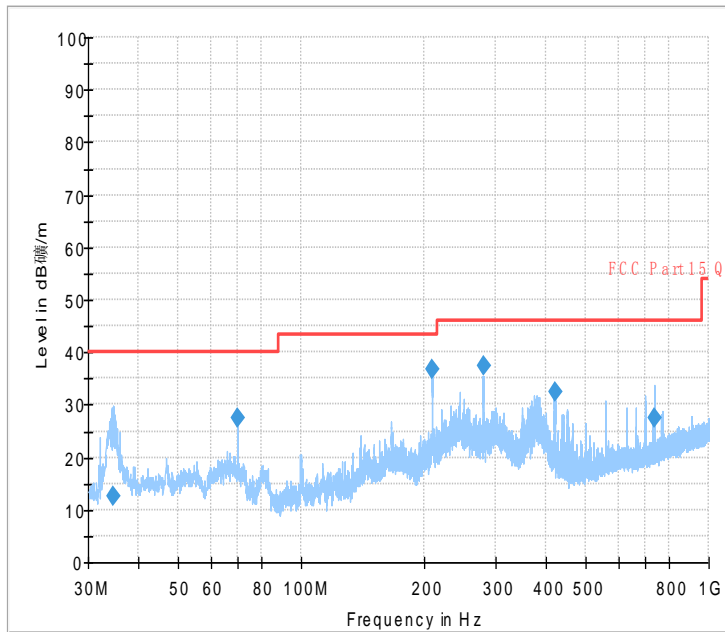
Fig.38 Radiated Spurious Emission (802.11g,Ch11,30MHz~1GHz)
