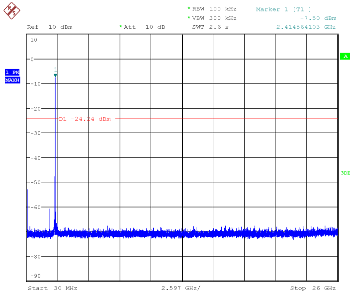
Fig.25 Conducted Spurious Emission (802.11n-20MHz, Ch1)
