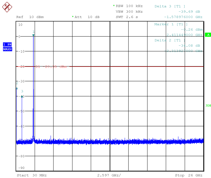
Fig.13 Conducted Spurious Emission (802.11b, Ch1)
