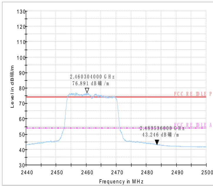
Fig.37 Radiated emission (Power): 802.11g, high channel
