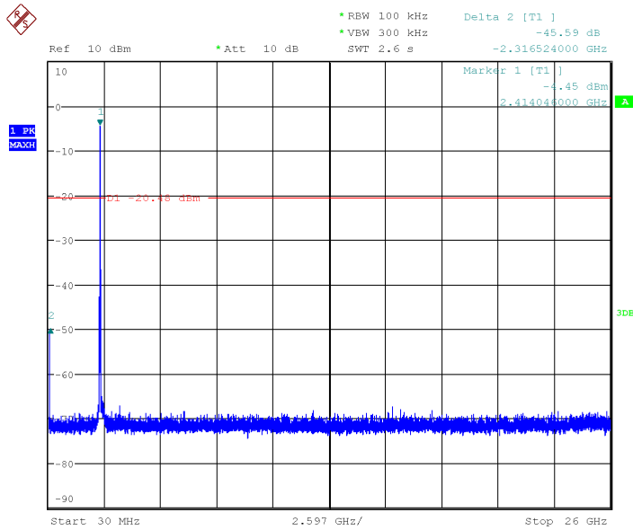
Fig.19 Conducted Spurious Emission (802.11g, Ch1)
