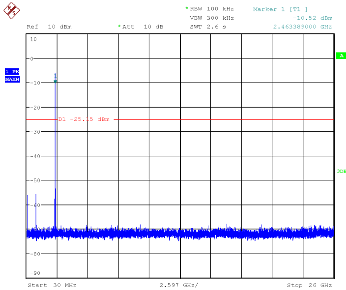
Fig.29 Conducted Spurious Emission (802.11n-20MHz, Ch11)
