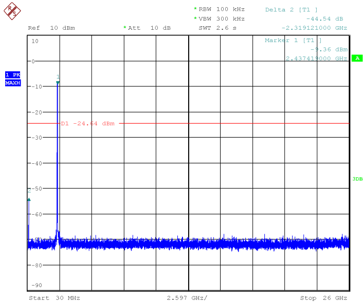
Fig.21 Conducted Spurious Emission (802.11g, Ch6)
