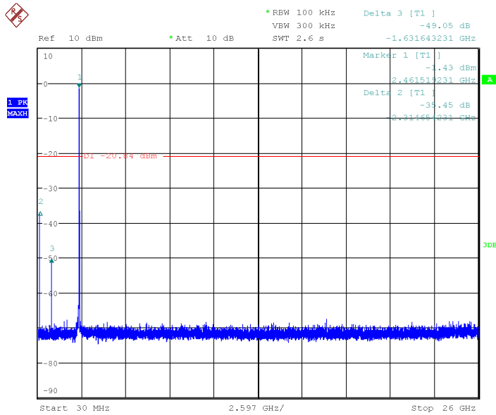
Fig.17 Conducted Spurious Emission (802.11b, Ch11)
