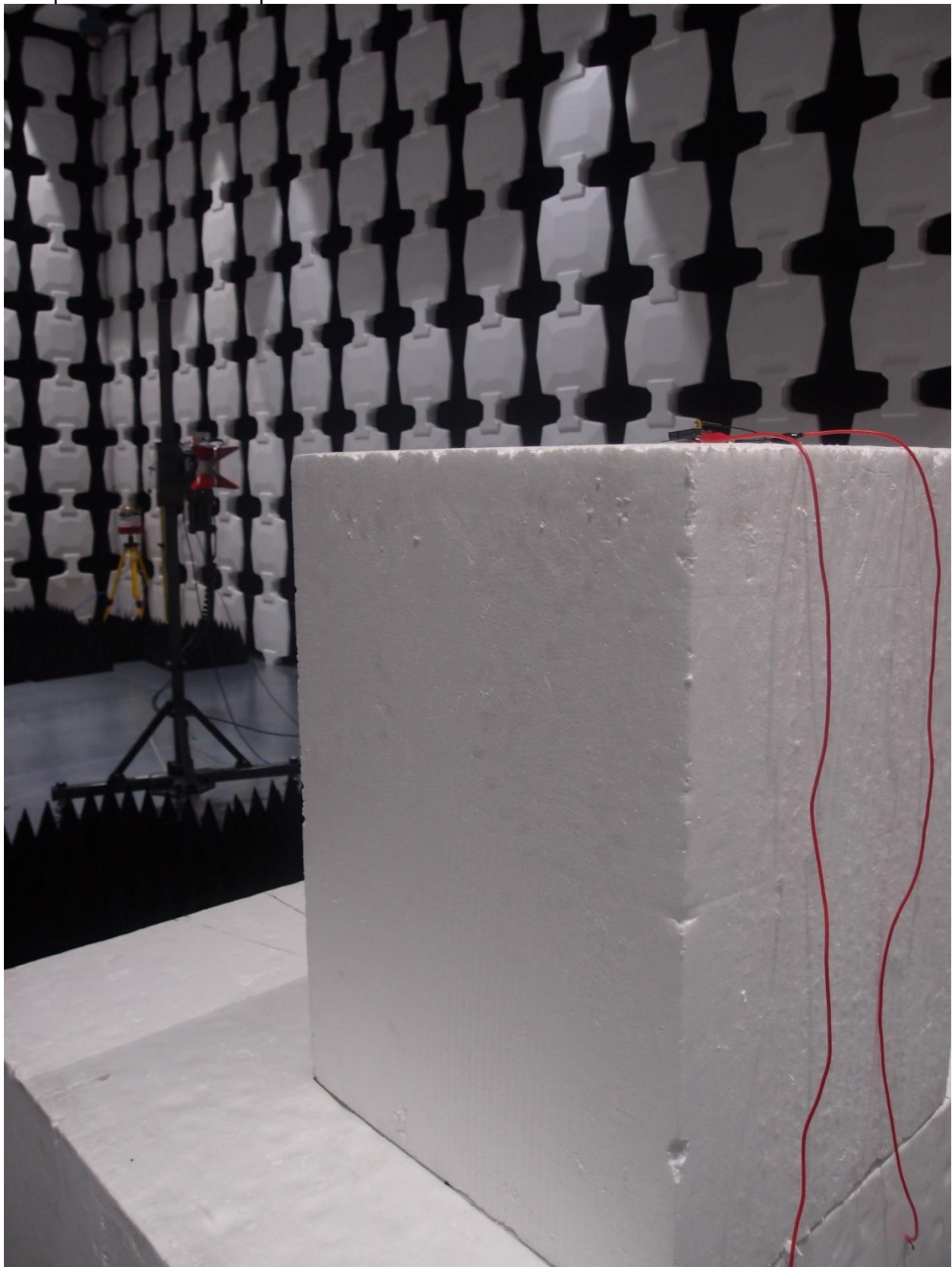
Description: EIRP Test Setup
