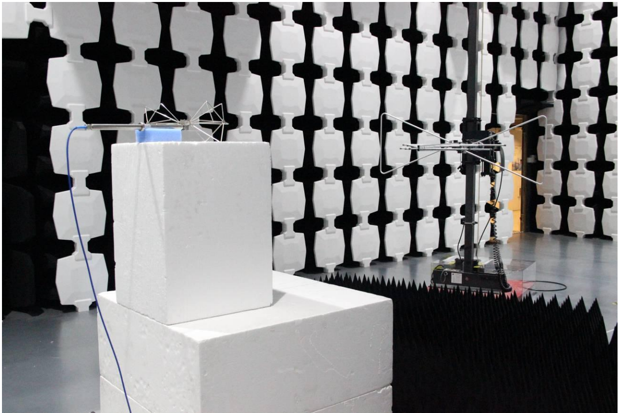
Description: Substitution Antenna for ERP Test
