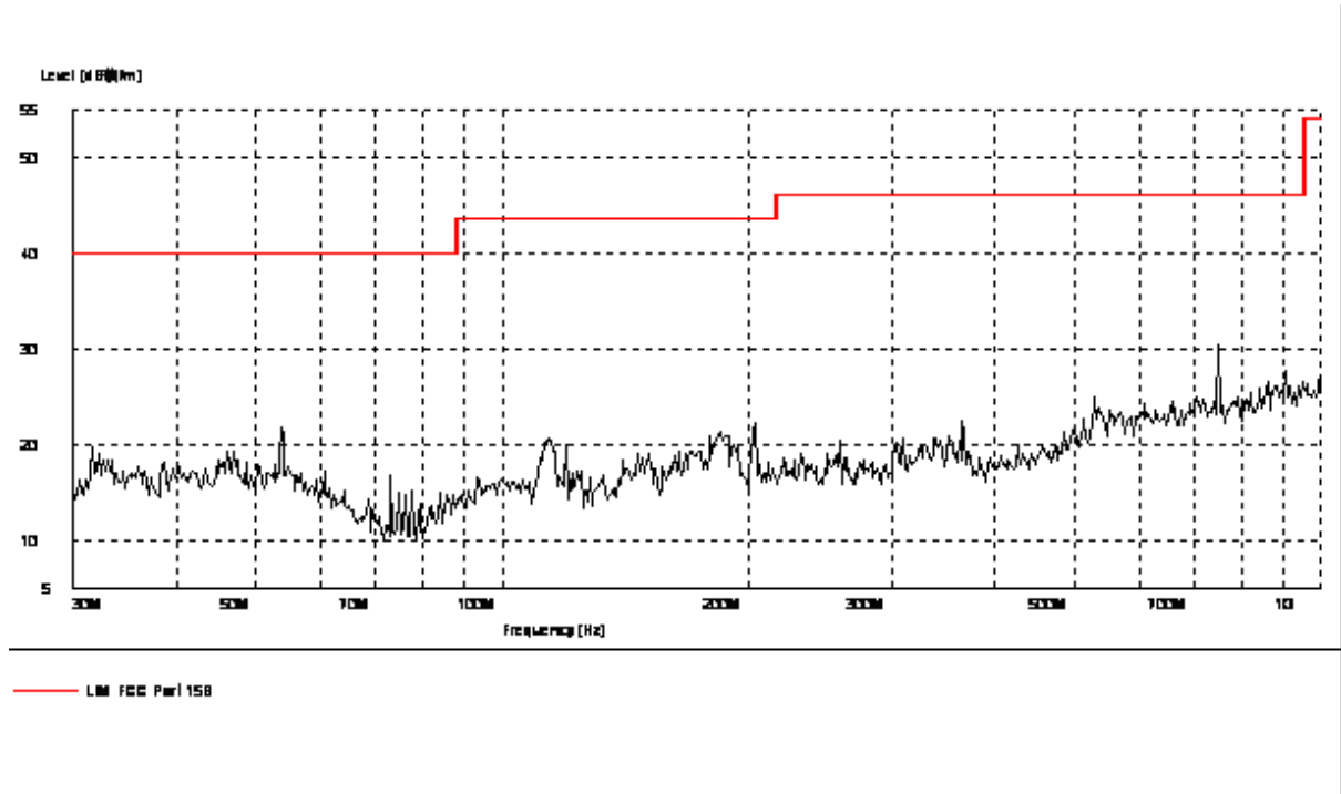
(WCDMA Band V: 30MHz-1GHz)
