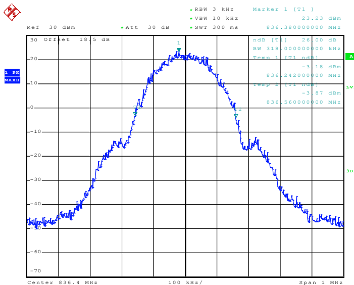
26dB Bandwidth Plot on Channel 189
