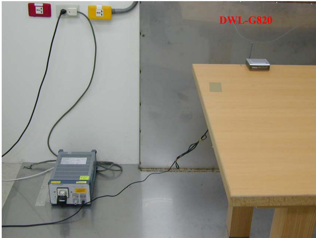
Photo 1: Conducted Emission Test Set-up
