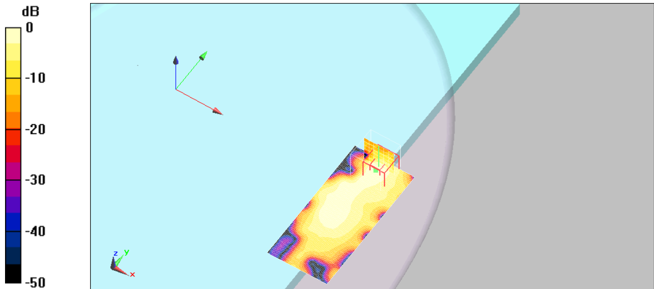
0 dB = 0.014mW/g
