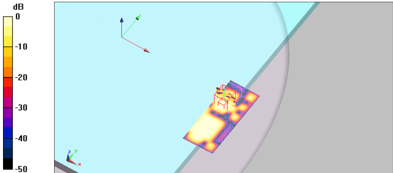
0 dB = 0.029mW/g
