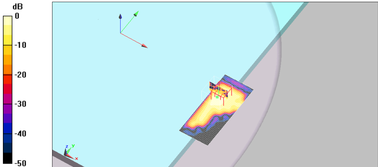
0 dB = 0.075mW/g
