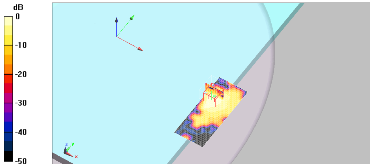
0 dB = 0.094mW/g
