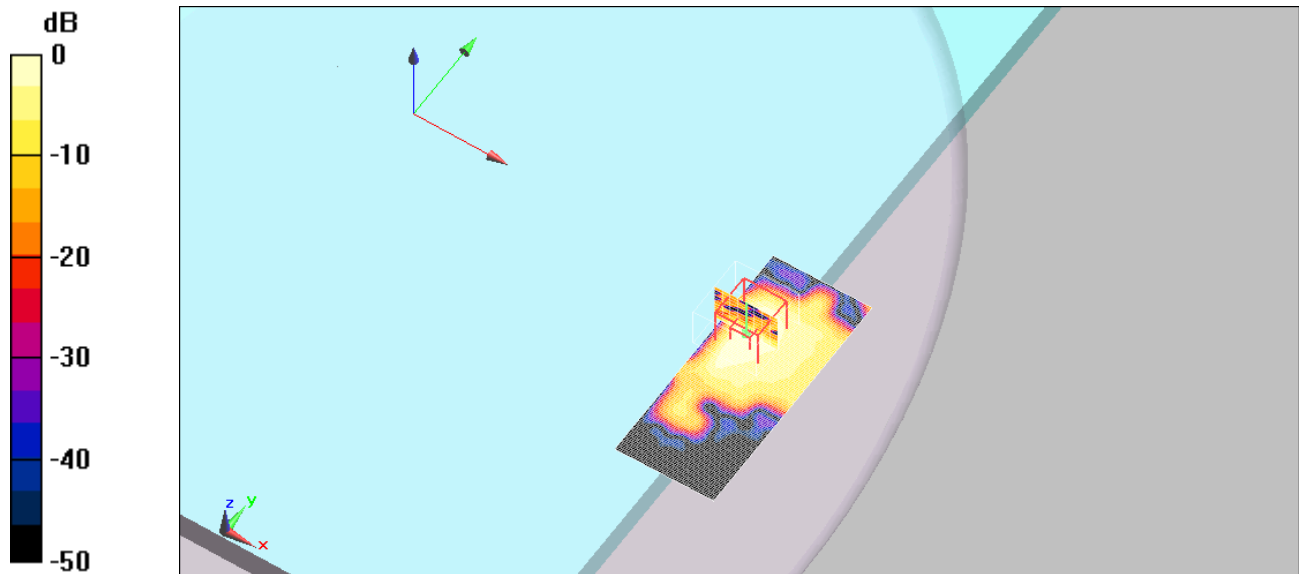
0 dB = 0.095mW/g
