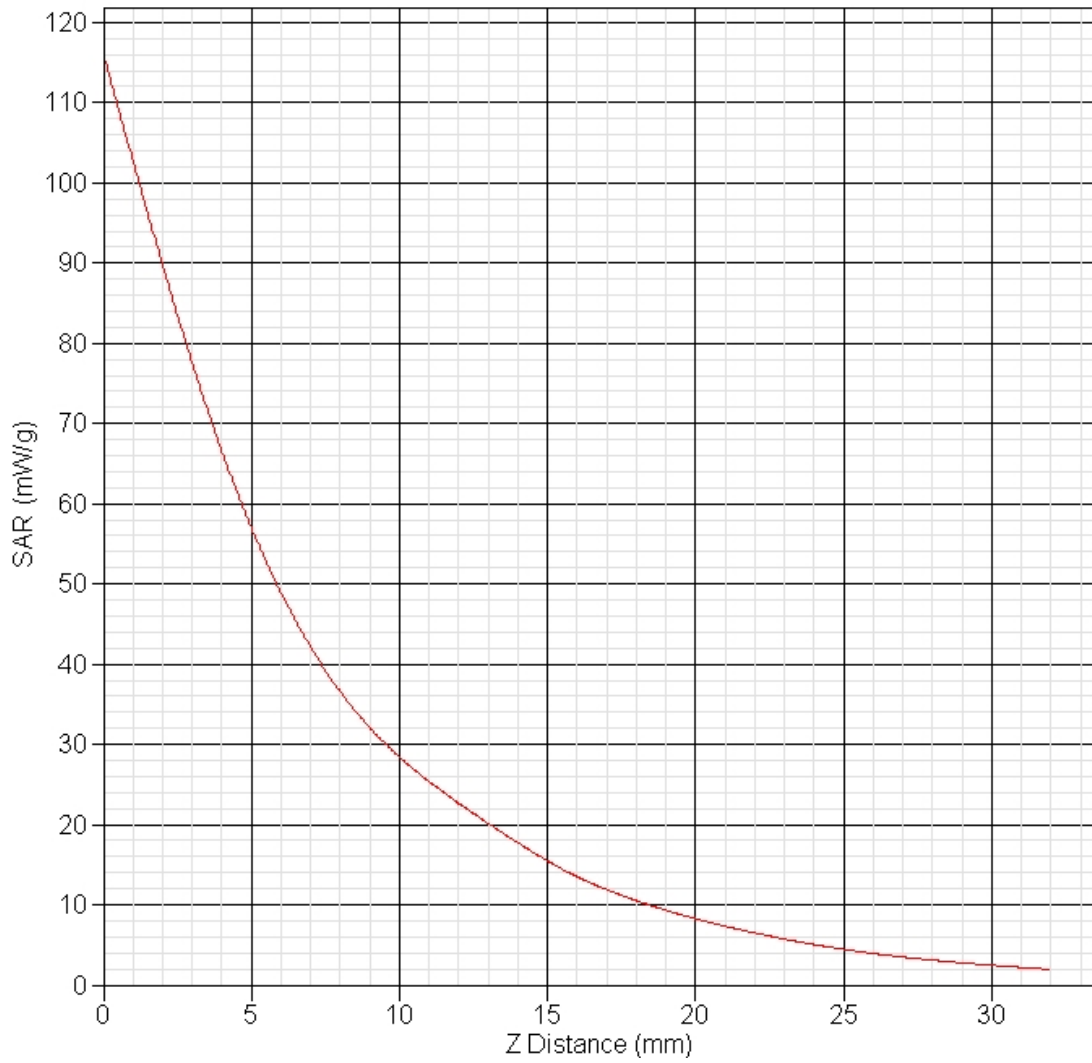
SAR-Z Axis at Hotspot x:0.02 y:-0.01
