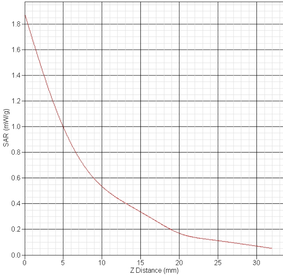
SAR-Z Axis at Hotspot x:-5.94 y:-0.01
