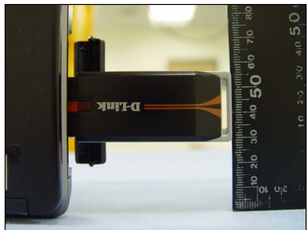
Distance is 28mm for Side(Edge)Touch
