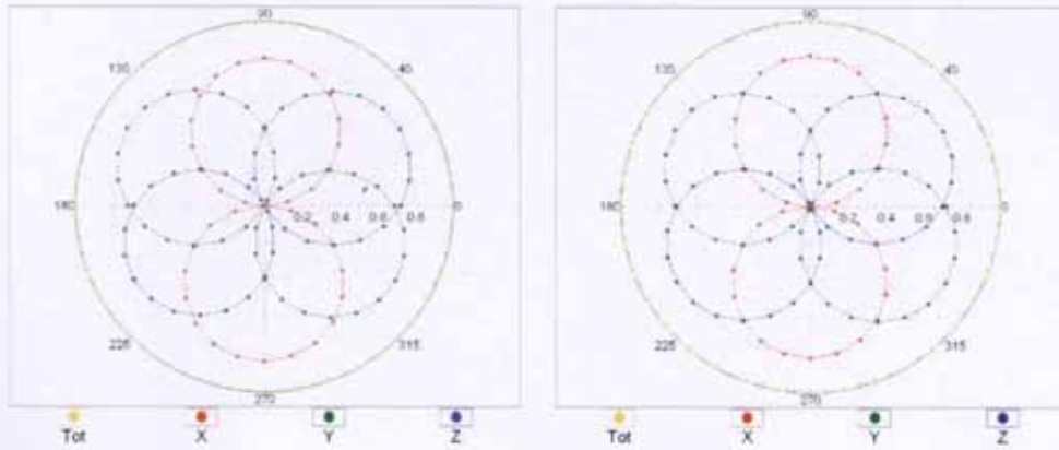
f=600 MHz,TEM
