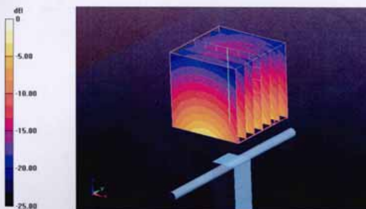
0 dB = 16.830mW/g
