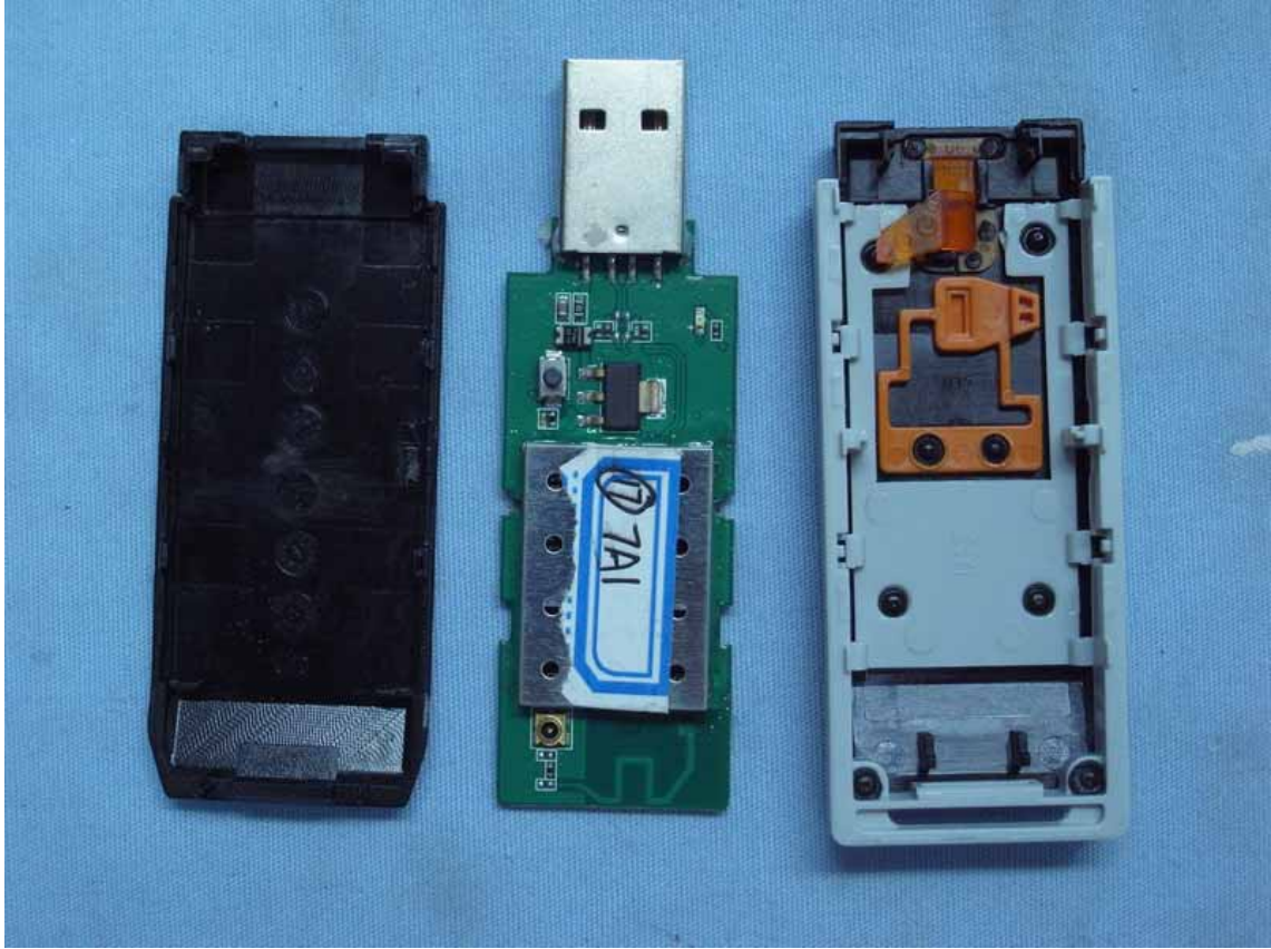
Figure 1 Inside of the EUT
