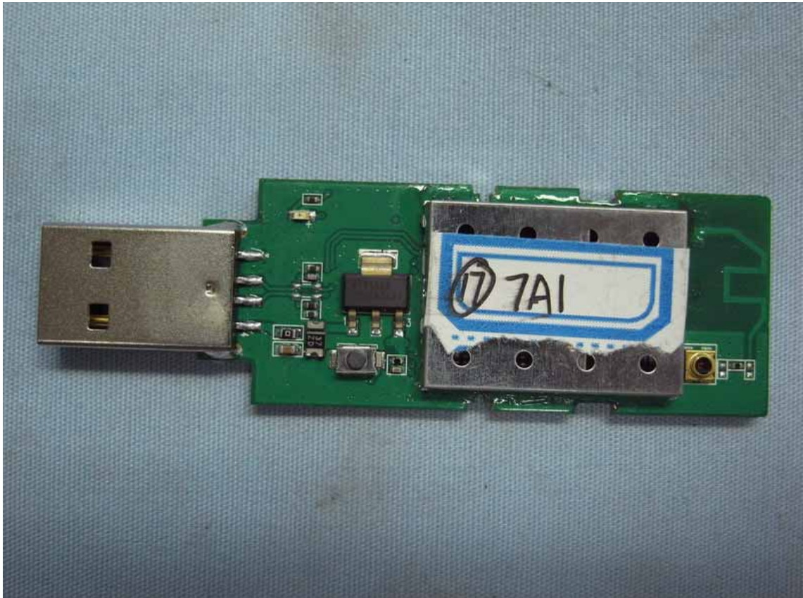
Figure 2 Inside of the EUT
