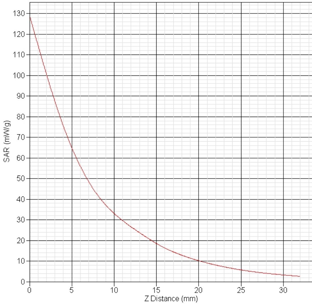
SAR-Z Axis at Hotspot x:0.17 y:-0.01
