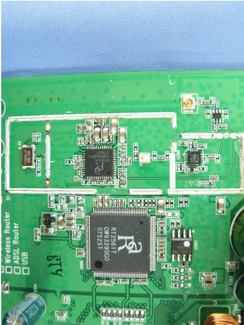
(26) EUT Photo
