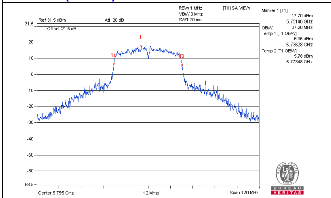
802.11ac (VHT40) / Chain 0 : CH151
