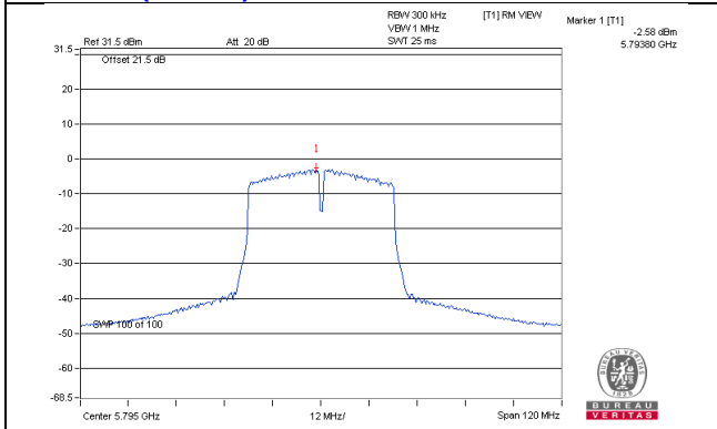
802.11ac (VHT40) / Chain 0: CH159
