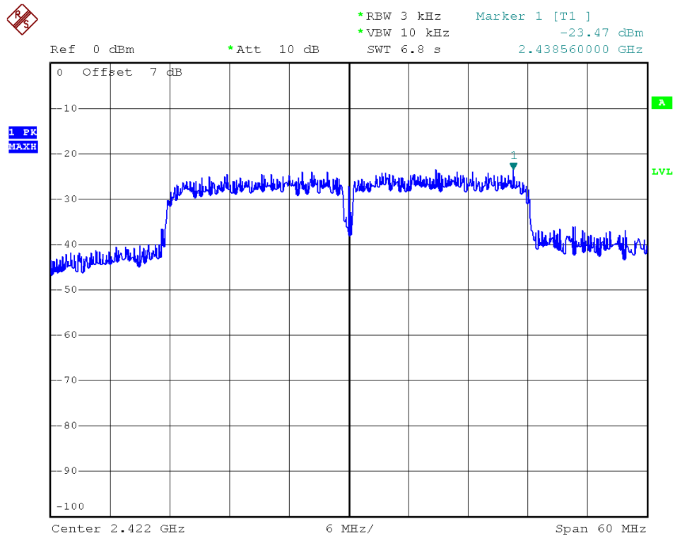
Channel 03 (2422MHz)
