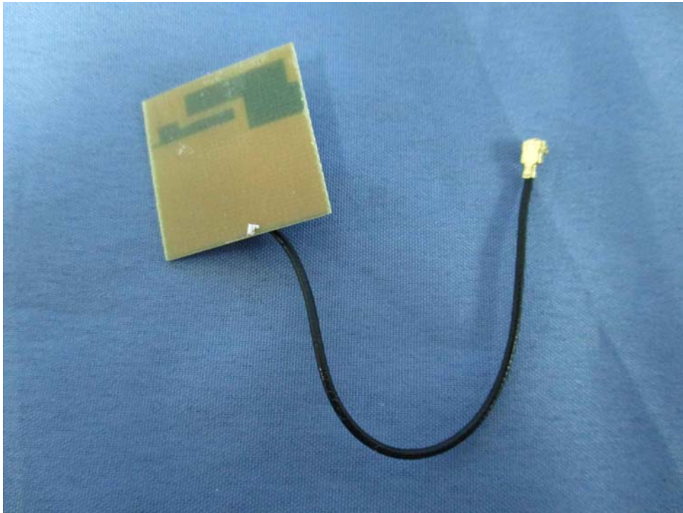
(24) EUT Photo (PCB Antenna)
