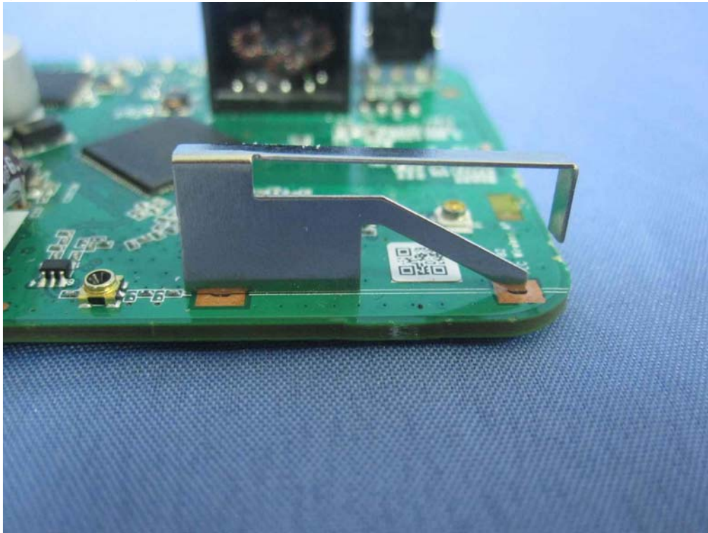
(22) EUT Photo (PIFA Antenna)
