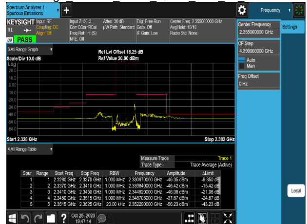
Band Edge Band40 5MHz QPSK RB1 24 CH39225
