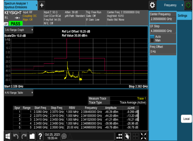
Band Edge Band40 5MHz QPSK RB1 0 CH39200
