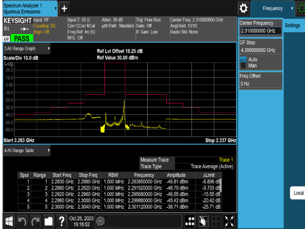
Band Edge Band40 5MHz QPSK RB1 24 CH38750
