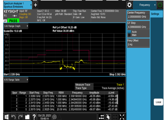
Band Edge Band40 5MHz QPSK RB1 0 CH39225
