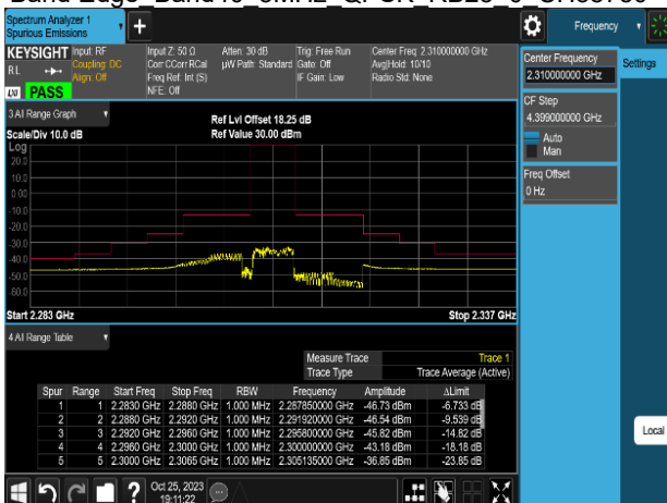
Band Edge Band40 5MHz QPSK RB25 0 CH38775
