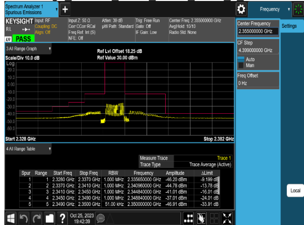
Band Edge Band40 5MHz QPSK RB25 0 CH39200
