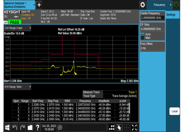
Band Edge Band40 5MHz QPSK RB1 24 CH39200
