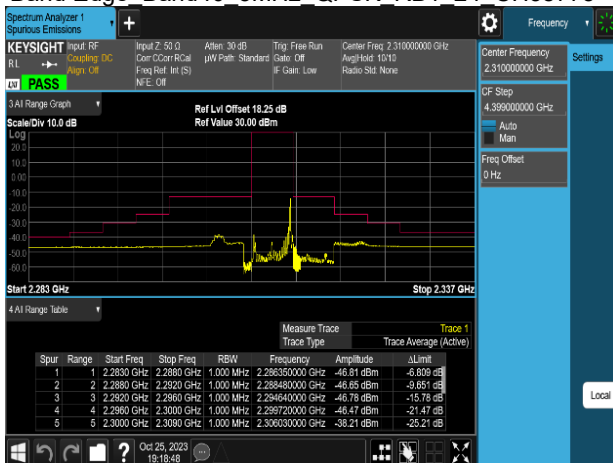
Band Edge Band40 5MHz QPSK RB1 24 CH38775
