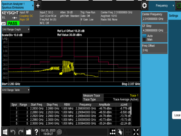
Band Edge Band40 5MHz QPSK RB25 0 CH38750
