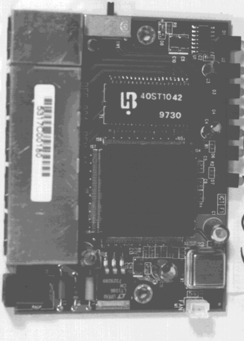
FCC ID: KA2ED4904H1 Front side of main board
