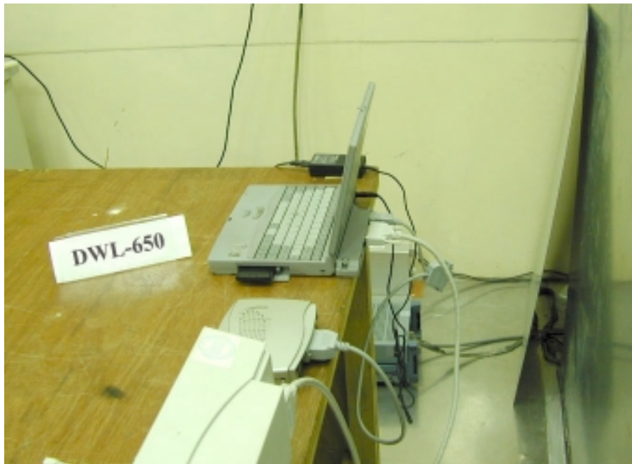
Photo 2: Conducted Test Set-up (rear)
