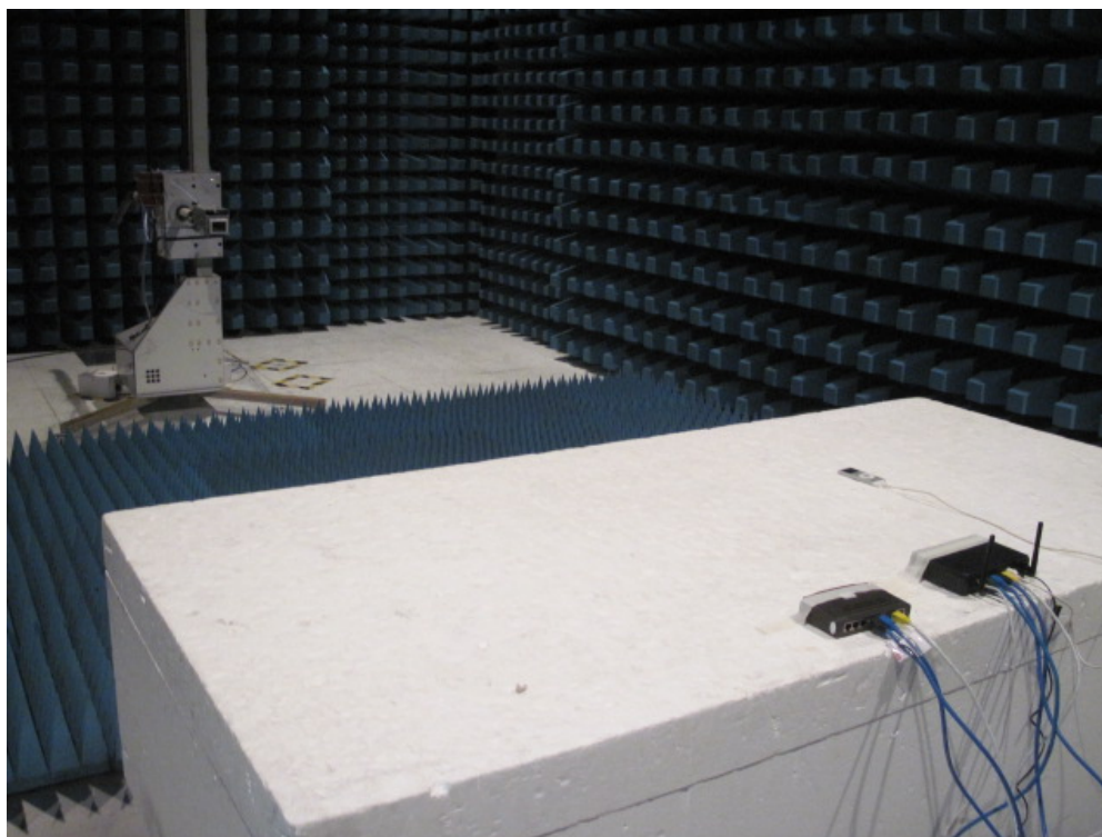
Description : Back View of Radiated Emission Test Setup for Above 18GHz
