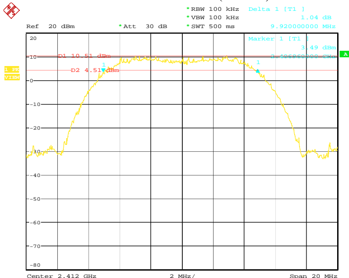
IEEE 802.11b 6dB Bandwidth (CH Low)
