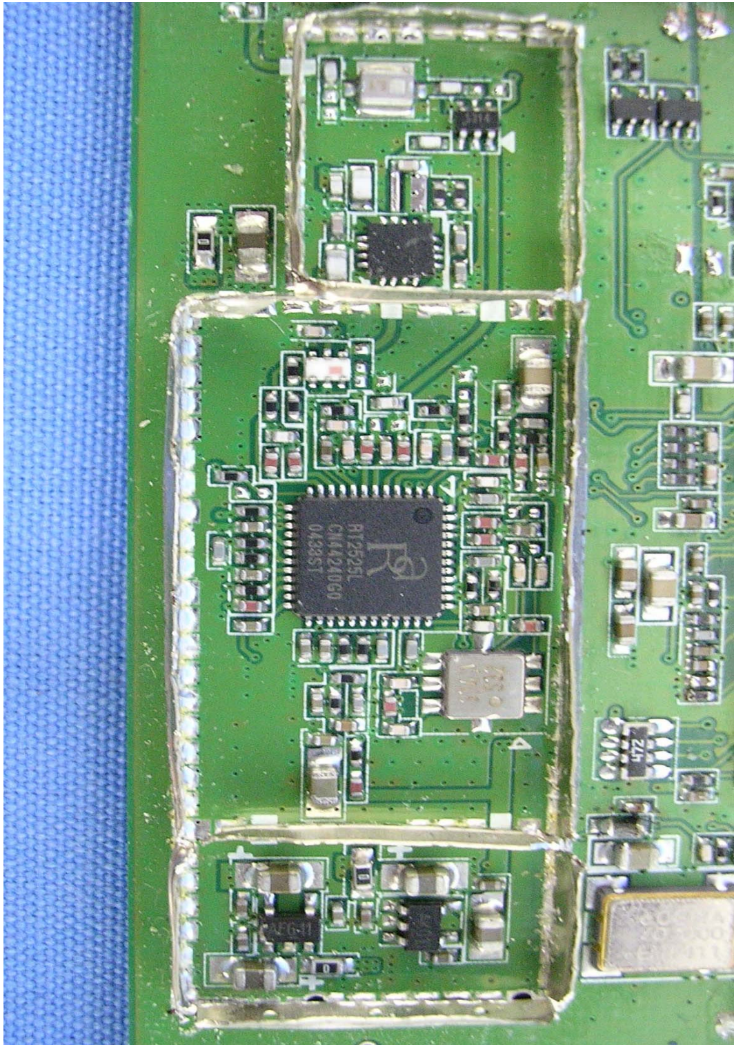
(11) EUT Photo
