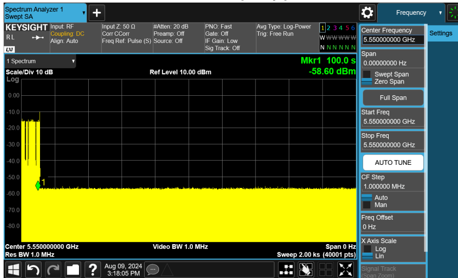
TX (IEEE 802.11n(HT40) Mode) 5550 Non-Occupancy period
