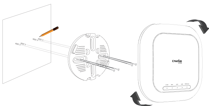
Figure 5: Attaching the Lock Plate
