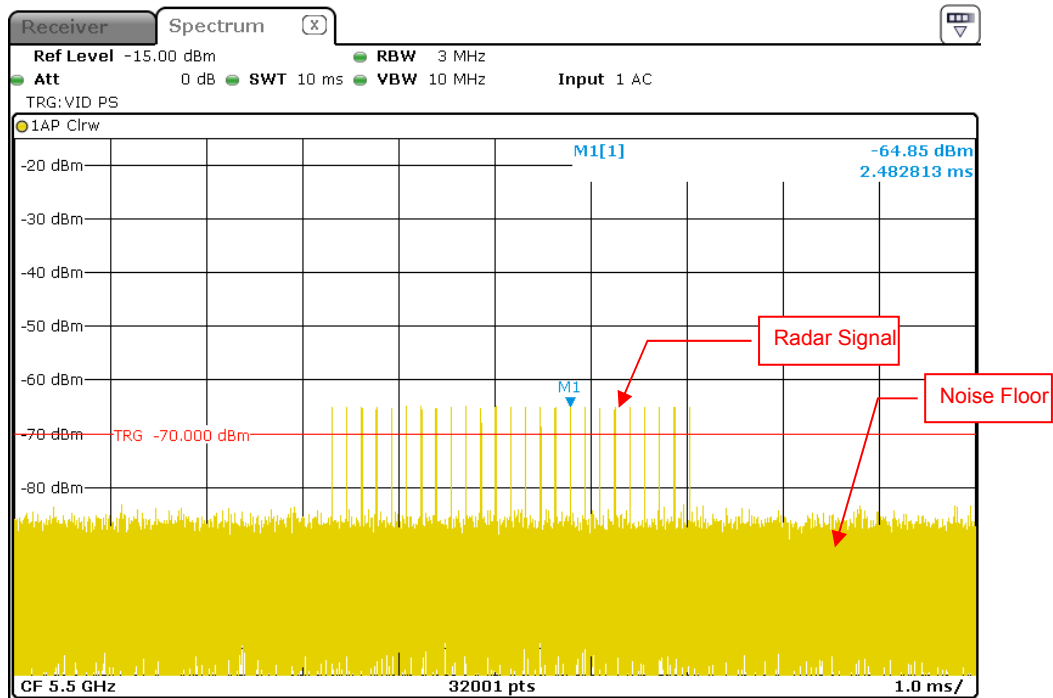
Radar Signal 2
