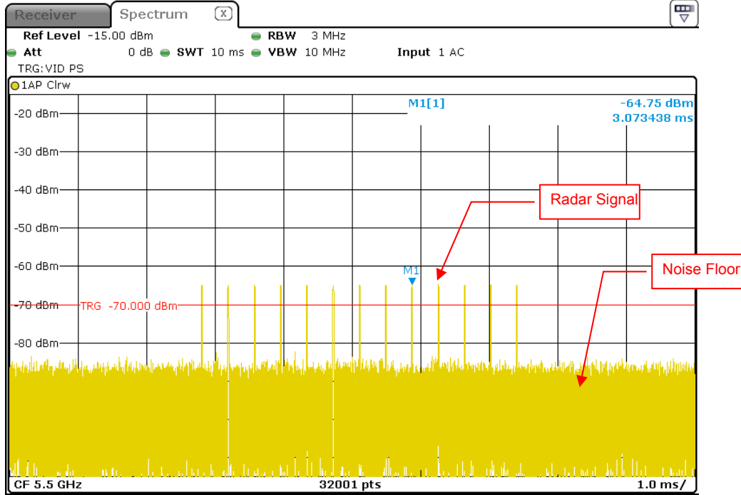
Radar Signal 4
