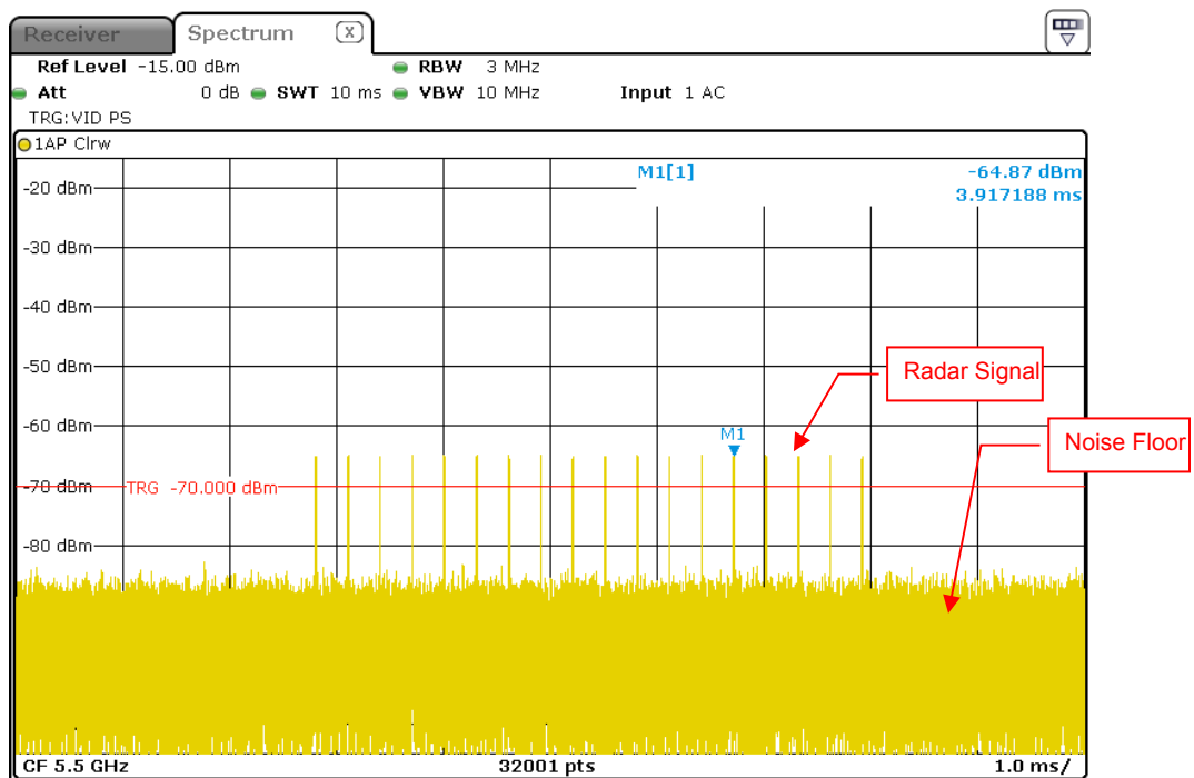
Radar Signal 3
