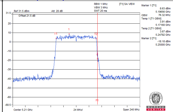
802.11ac(VHT80)_Chain0 / CH42
